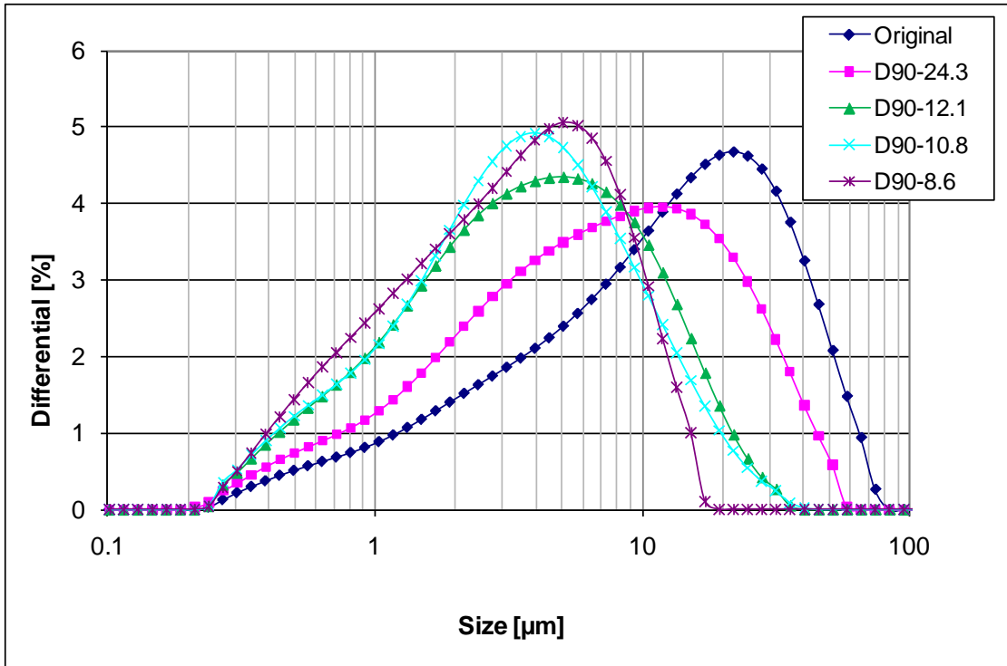
Figure 1. Particle size distributions of the five cements. Each shown result is the average of six individual measurements and the error bars (one standard deviation) would fall within the size of the shown symbols.
