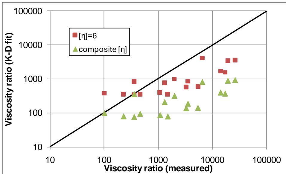
Figure 5. Viscosity ratios predicted by applying the K-D equation vs. those measured for the various cement/fly ash mixtures.
