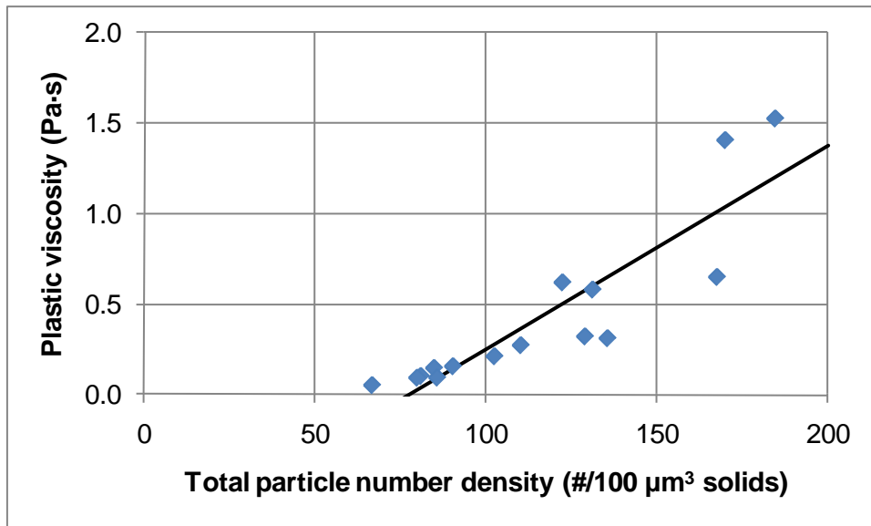
Figure 7. Measured plastic viscosity vs. total particle (number) density. Best fit ( R^2=0.792 ) is shown for all data with measured viscosities of less than 2 Pa-s.
