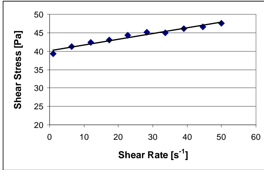
Figure 3. Typical descending branch shear stress vs. shear rate curve obtained for cement/fly ash paste mixture.
