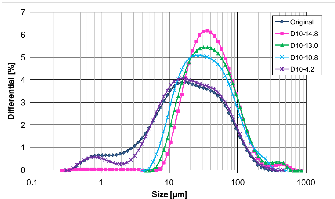
Figure 2. Particle size distributions of the five fly ashes. Each shown result is the average of six individual measurements and the error bars (one standard deviation) would fall within the size of the shown symbols.
