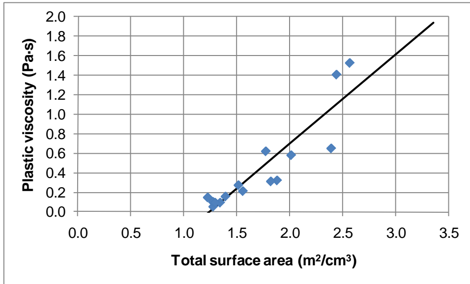
Figure 6. Measured plastic viscosity vs. total surface area. Best fit ( R^2=0.817 ) is shown for all data with measured viscosities of less than 2 Pa-s.
