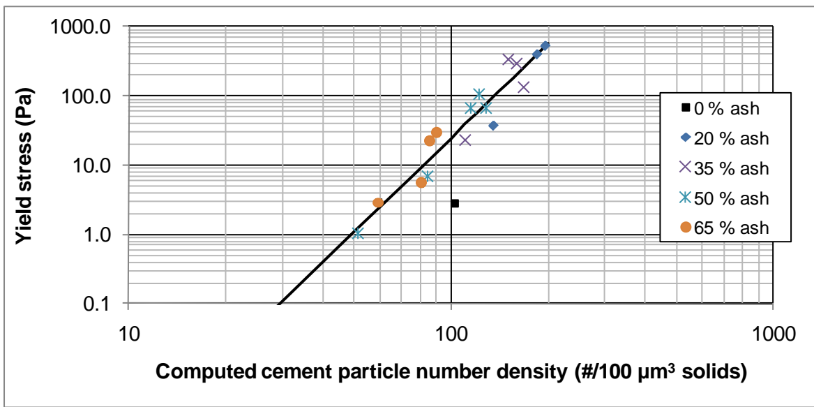
Figure 4. Log-log plot of yield stress vs. cement particle density. Best fit ( R^2=0.918 ) is shown for all of the data with the exception of the single 0 % fly ash data point.
